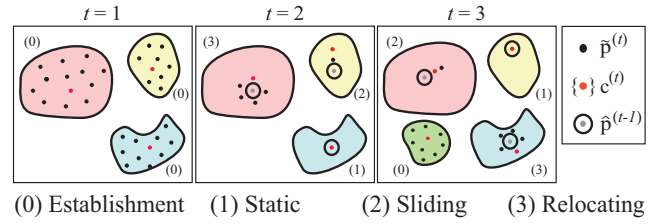
Figure 3: Each colored region indicates a surface patch for a finger. Three initial patches appear at t = 1 , and a fourth one appears at t = 3 . Contact points evolve on the patches over time according to strategies (0)-(3).
